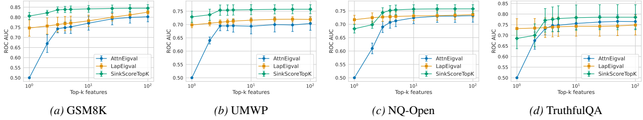
Figure 5. Influence of the hyperparameter k . Varying the number of retained sink scores per head, we find that SinkProbe attains best or near-best performance even for small values of k . This suggests that hallucination-related signals are concentrated in a few dominant sinks and that sink-score features capture this signal more directly and robustly than existing attention- or spectral-based representations. The presented results are for Llama3.2-3B, for other models and datasets see Section C.
